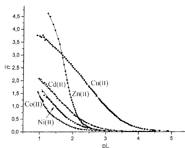
Fig. 1 Formation curves of 2-methyl-1-vinylimidazole complexes with \text{Co}^{2+} , \text{Ni}^{2+} , \text{Cu}^{2+} , \text{Zn}^{2+} and \text{Cd}^{2+} .
